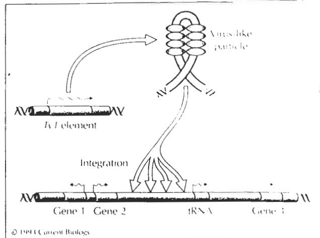
Fig. 1. Integration-target selection by the yeast retrotransposon Ty1 . Transcription from a pre-existing Ty1 element, followed by complex formation with viral proteins and reverse transcription, yields a virus-like particle. Integration occurs preferentially in non-protein-coding sequences upstream of tRNA genes. Integration events are rare in the coding regions of cellular genes, despite the fact that 70% of the target chromosome is coding region.
